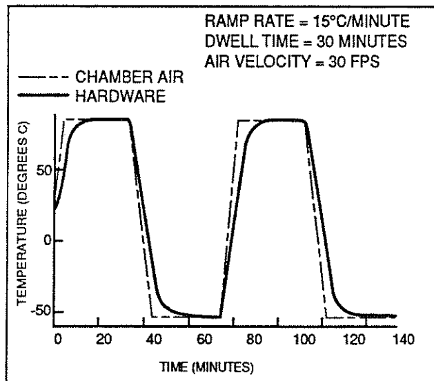
FIGURE 5-1. TEMPERATURE HISTORIES WITH HIGH CHAMBER AIR SPEED AND LONG DWELL TIMES
