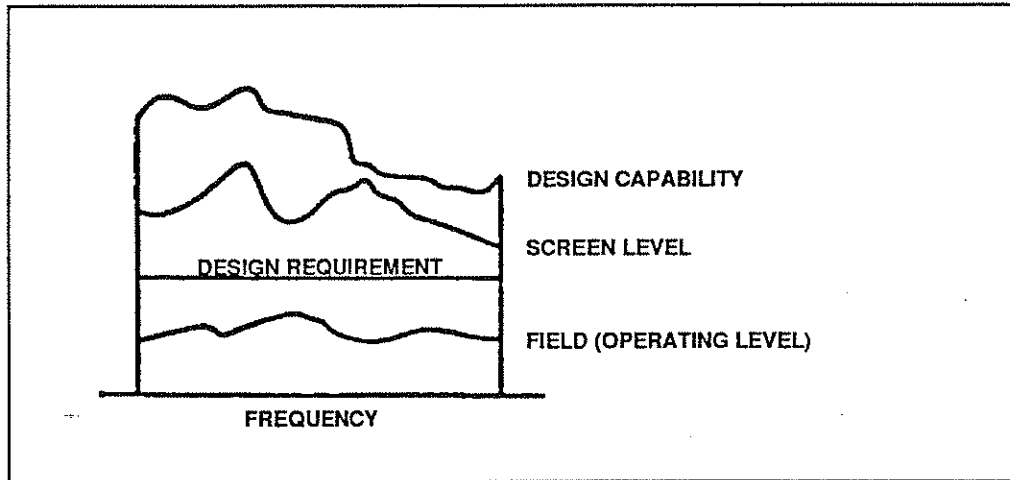
FIGURE 4-3. STEP-STRESS CONCEPT: RELATION OF ENVIRONMENTAL LEVELS
