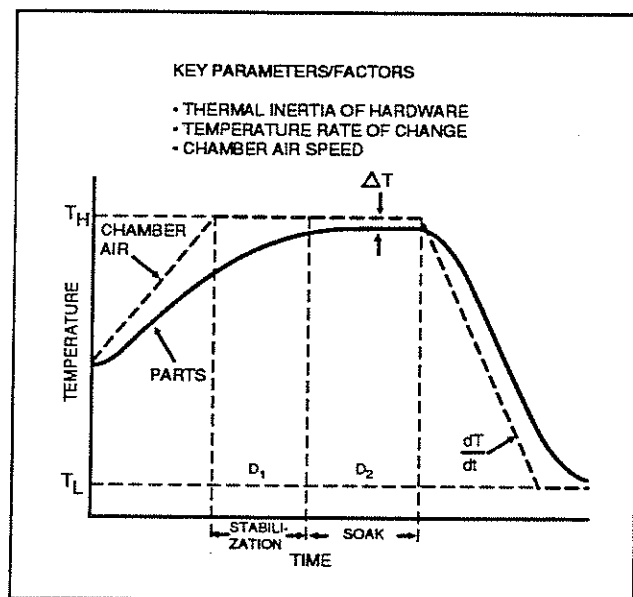
FIGURE 5-3. TYPICAL TEMPERATURE CYCLING PROFILES
